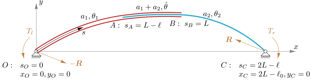
Figure 4: Flexible rod (sub-rod 2, blue) partially inserted in a flexible sleeve (sub-rod 1, red) with transition points A and B and imposed distance between the two supports in O and C defined as 2L - \ell_0 > L . The externally applied bending moments T_l and T_r , as well as the reaction forces \mathbf{R} and -\mathbf{R} , are plotted at the hinged end points. The presented shape is the equilibrium solution for a_1 = 1.5 , a_2 = 1 , L = 1 , \ell_0 = 0.5 , and T_l = T_r = 1 (SI units) computed using the code presented in Fig. 7.
