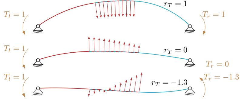
Figure 13: Deformed shapes and distribution of normal contact force for different moment ratios r_T = \{-1.3, 0, 1\} , see Section 6.5. The normal force distribution changes direction when the moment is reduced at the right end, and the force vanishes at the inflection point when r_T = -1.3 . Note that, for simplicity of representation, only the contact force distribution is plotted, while the concentrated interaction forces and moments at the transition points are not represented.
